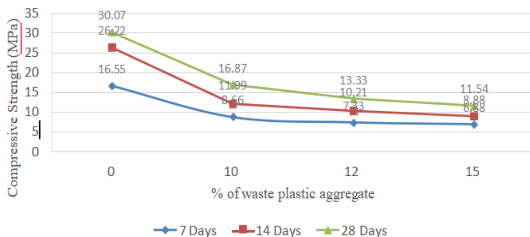
Fig. 4 Compressive strength curve for cubes with varying percentages
