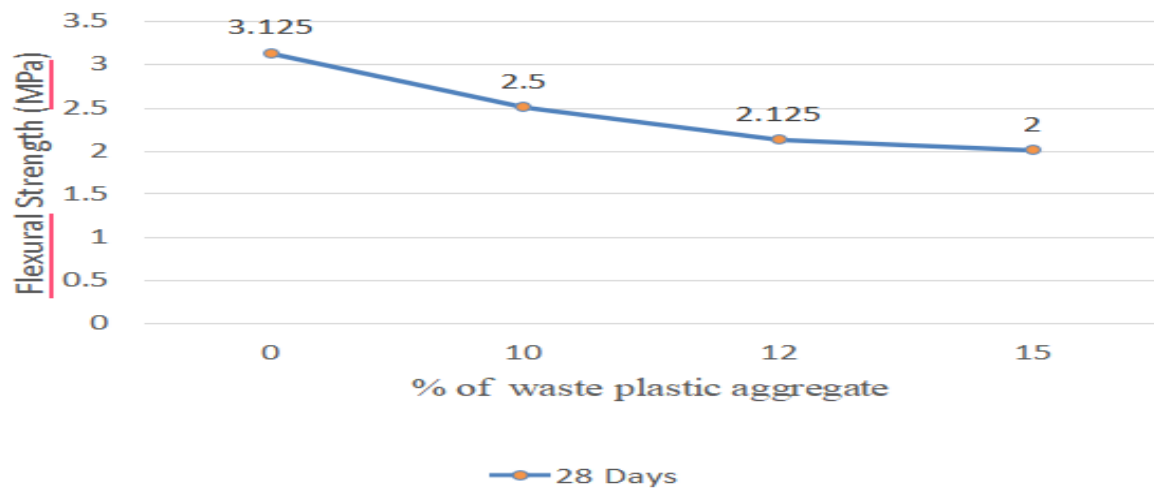
Fig 5. Flexural strength curve of the beam
