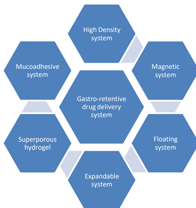
Fig. 2. Gastro-retentive drug delivery system based on high density.
