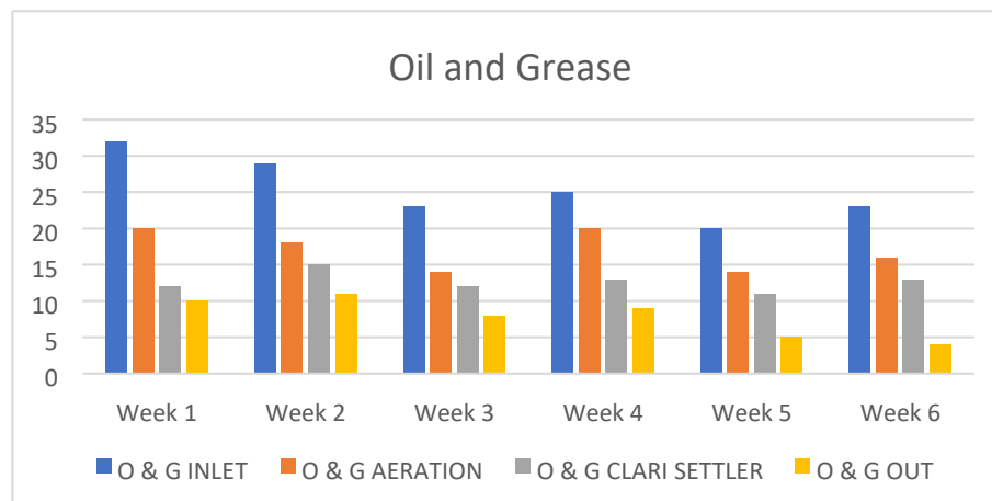
Fig 8 Performance analysis of Oil and Grease
