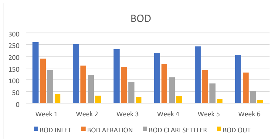
Figure 4 Performance analysis of Bio-chemical oxygen Demand
