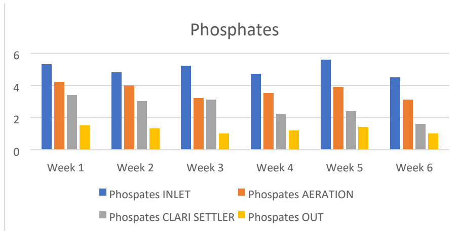
Fig 9 Performance analysis of Phosphates
