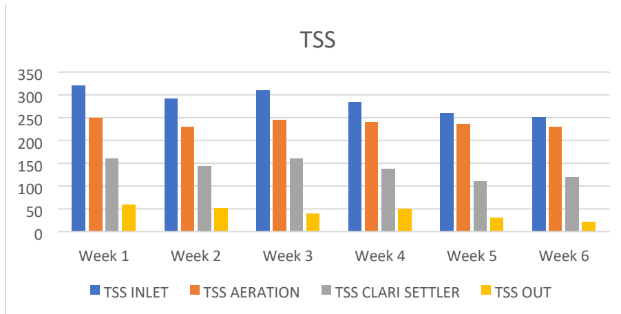
Fig 6 Performance analysis of Total Suspended Solids
