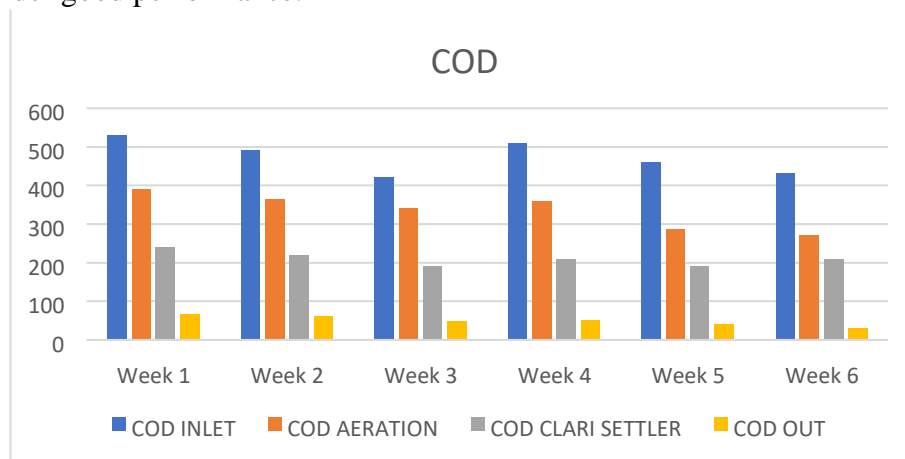
Figure 5. Performance analysis of Chemical oxygen Demand
