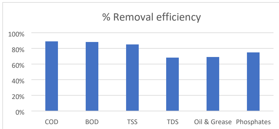
Fig 10 Overall % Removal Efficiency of the Plant
