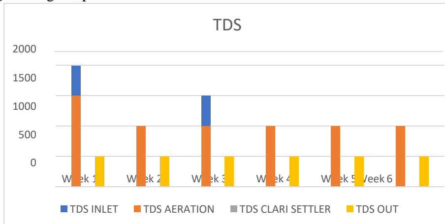
Fig 7 Performance analysis of Total Dissolved Solids
