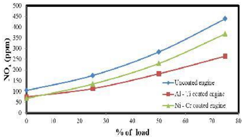
Figure 6: Comparison of Oxides of Nitrogen emission for different loads.
