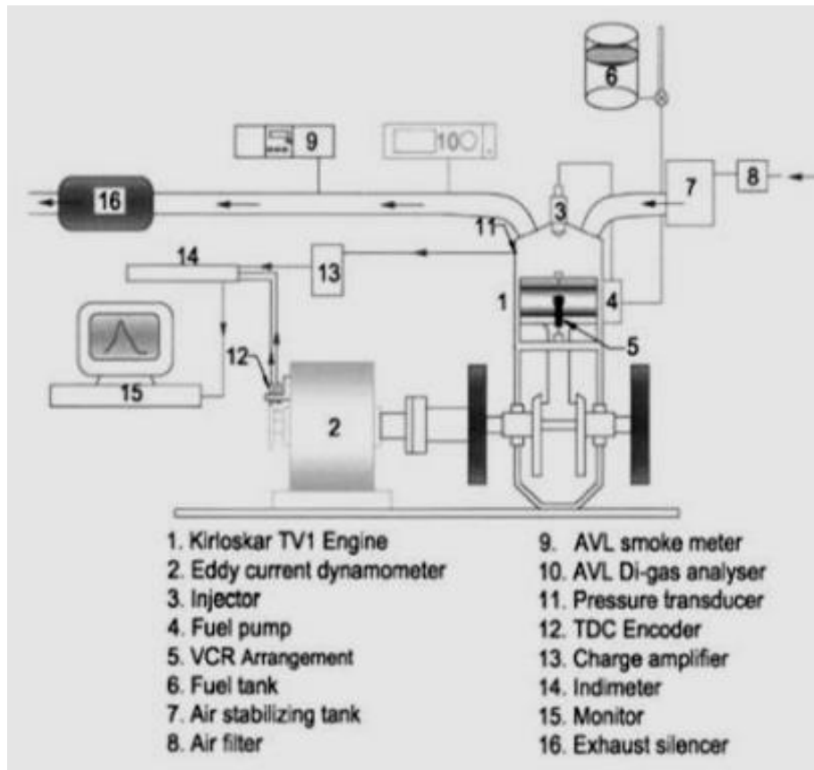
Figure 1: Schematic view of experimental set- up
