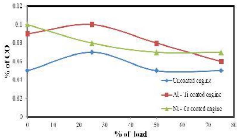
Figure 7: Comparison of carbon monoxide emission for different loads.
