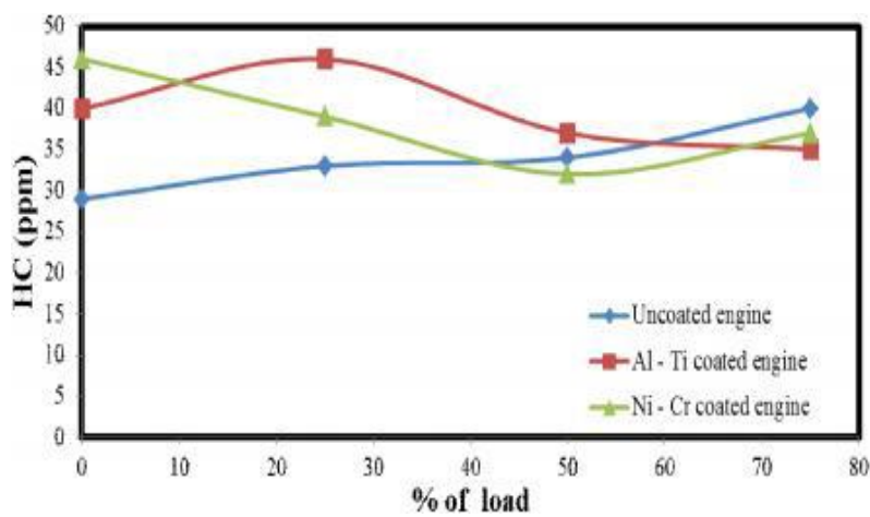
Figure 5: Comparison of Hydrocarbon emission for different loads.
