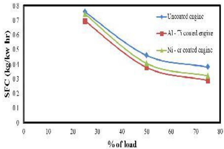
Figure 3: Comparison of Specific Fuel consumption for different loads.
