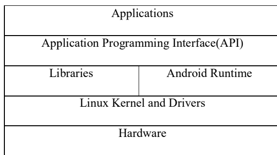
Android Architecture [2]
